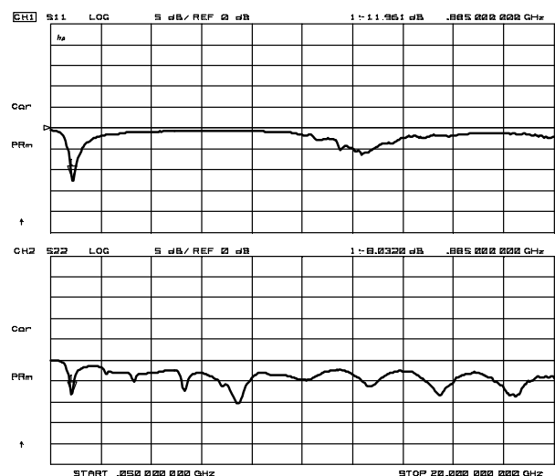
S11, S22
