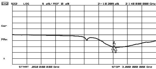
S11, S22
