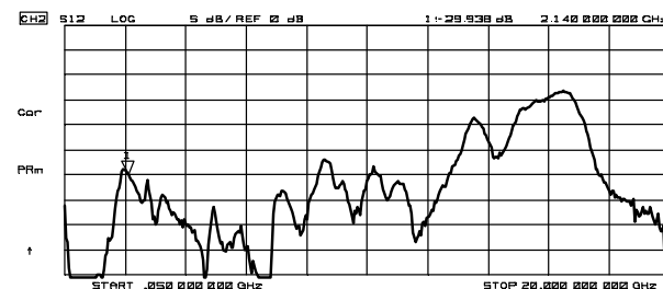
S21, S12 (f=50MHz~20GHz)
