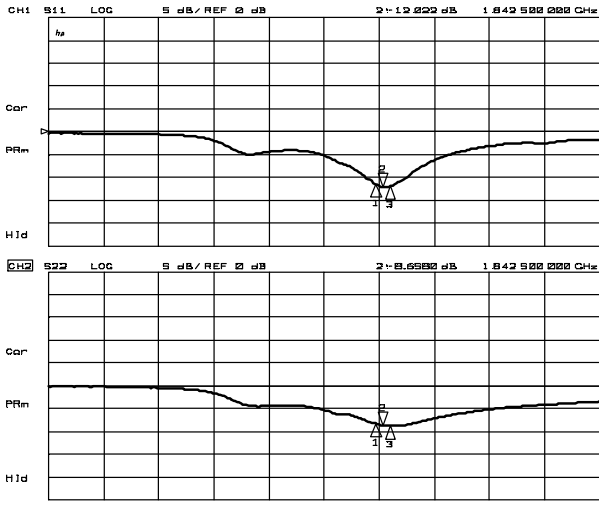
S11, S22
