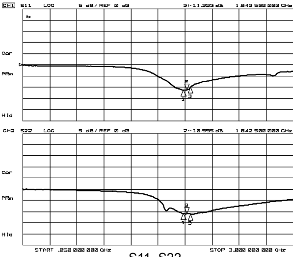
S11, S22
