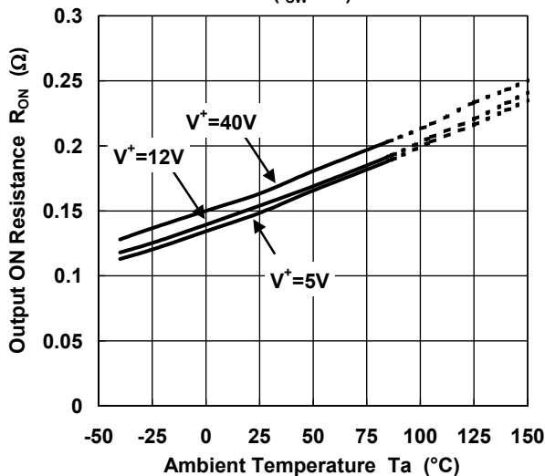
Output ON Resistance vs. Temperature ( I_{sw}=3A )
