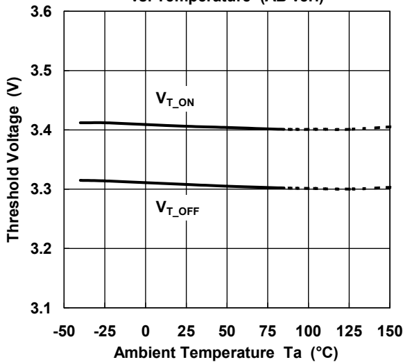
Under Voltage Lockout Voltage vs. Temperature (AB ver.)
