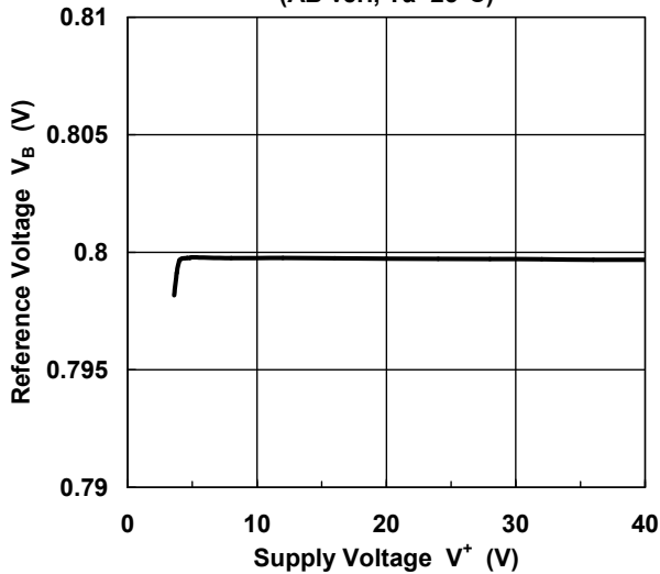
Reference Voltage vs. Supply Voltage (AB ver., T_a=25^\circ C )
