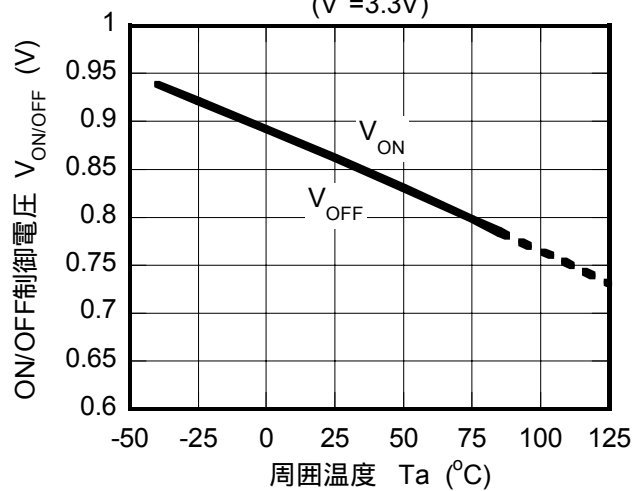
ON/OFF制御電圧温度特性例 ( V^+=3.3V )
