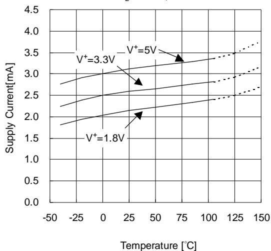
Supply Current vs Temperature [STANDBY]
