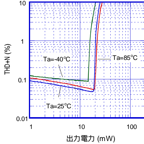
THD+N 对 出力電力特性例 ( V_+ = 2.8V, f = 1KHz, RL = 16\Omega )
