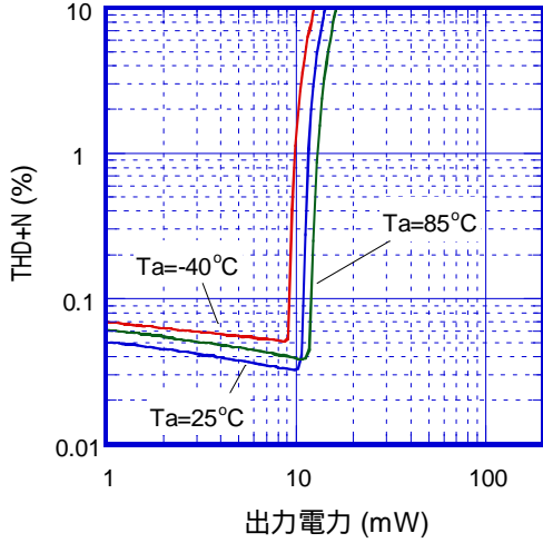
THD+N 对 出力電力特性例 ( V_+ = 2.8V, f = 1KHz, RL = 32\Omega )
