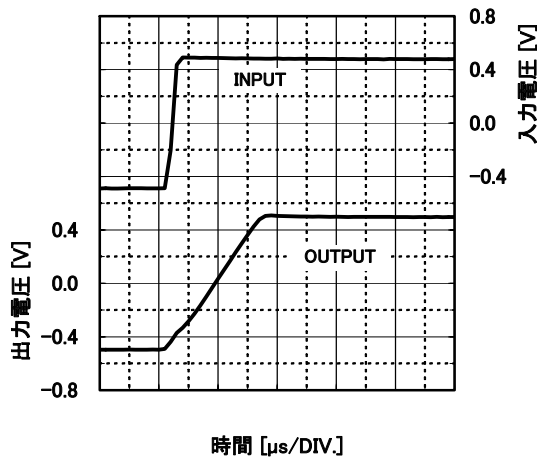
パルス応答特性例 (上昇時) V^+ / V^- = \pm 1.5V, G_v = 0dB, f = 10kHz, V_{IN} = 1V_{PP} R_S = 50\Omega, R_L = 2k\Omega, C_L = 0pF, T_a = +25^\circ C
