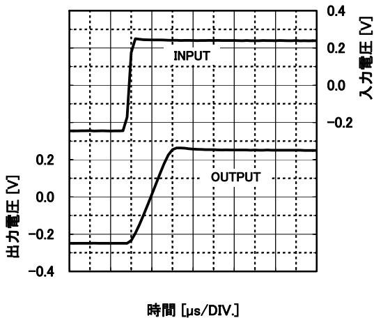
パルス応答特性例 (上昇時) V^+ / V^- = \pm 0.9V, G_v = 0dB, f = 10kHz, V_{IN} = 0.5V_{PP} R_S = 50\Omega, R_L = 2k\Omega, C_L = 0pF, T_a = +25^\circ C
