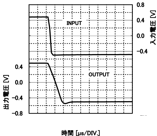
パルス応答特性例 (下降時) V^+ / V^- = \pm 1.5V, G_v = 0dB, f = 10kHz, V_{IN} = 1V_{PP} R_S = 50\Omega, R_L = 2k\Omega, C_L = 0pF, T_a = +25^\circ C
