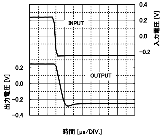
パルス応答特性例 (下降時) V^+ / V^- = \pm 0.9V, G_v = 0dB, f = 10kHz, V_{IN} = 0.5V_{PP} R_S = 50\Omega, R_L = 2k\Omega, C_L = 0pF, T_a = +25^\circ C
