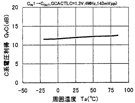
C系電圧利得対周囲温度特性例 (V'1=4.8V, V'2=3.0V, CIN1 → COUT, GCACTL C=1.3V, 4MHz, 143mVpp)
