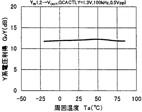
Y系電圧利得対周囲温度特性例 (V'1=4.8V, V'2=3.0V, YIN1,2 → VOUT, GCACTL Y=1.3V, 100kHz, 0.5Vpp)
