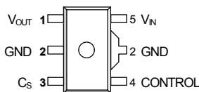
NJM12884U2
