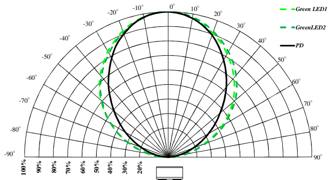
Directivity at Package direction Y
