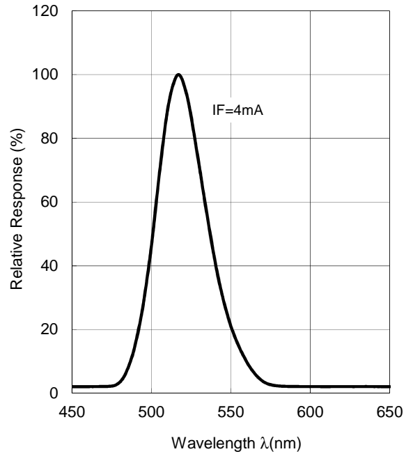
Spectral Response (Ta=25°C) Emitter GREEN LED
