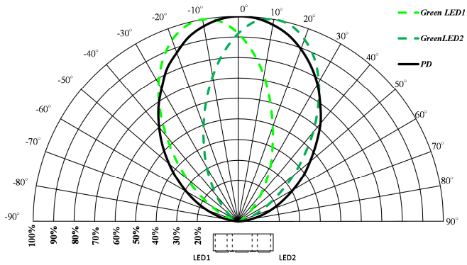
Directivity at Package direction X
