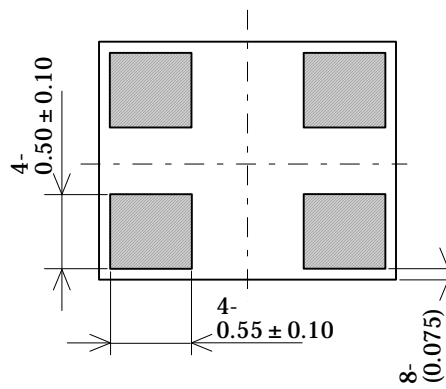
Fig.2 Package dimensions (in mm)
